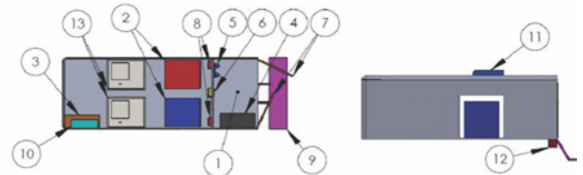
1) Workspace, 2) Spare Totes, 3) Toolbox-workbench, 4) Compressor-Generator, 5) Pumps, 6) M7 Monitoring System, 7) Hose Hanger, 8) Heat Exchange, 9) Deck, 10) Cabinets, 11) AC/Heater, 12) Furnace, 13) Heated Tanks
